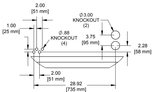
KNOCKOUT DETAIL
