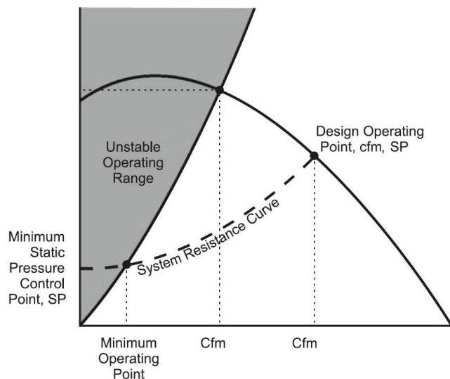
Figure 18: Variable Air Volume (VAV) Control
