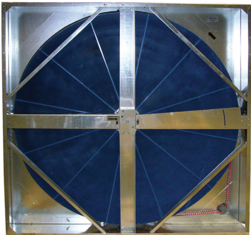
Figure 9: Energy Recovery Wheel
