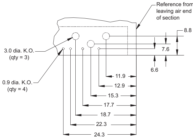
Figure 79: Main Control Panel/Discharge Plenum Knockout Detail
