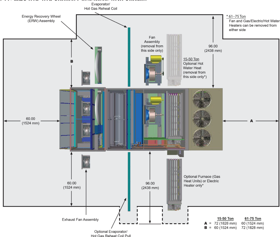
Figure 17: MPS 015–075 Service Clearances (020 Shown)
