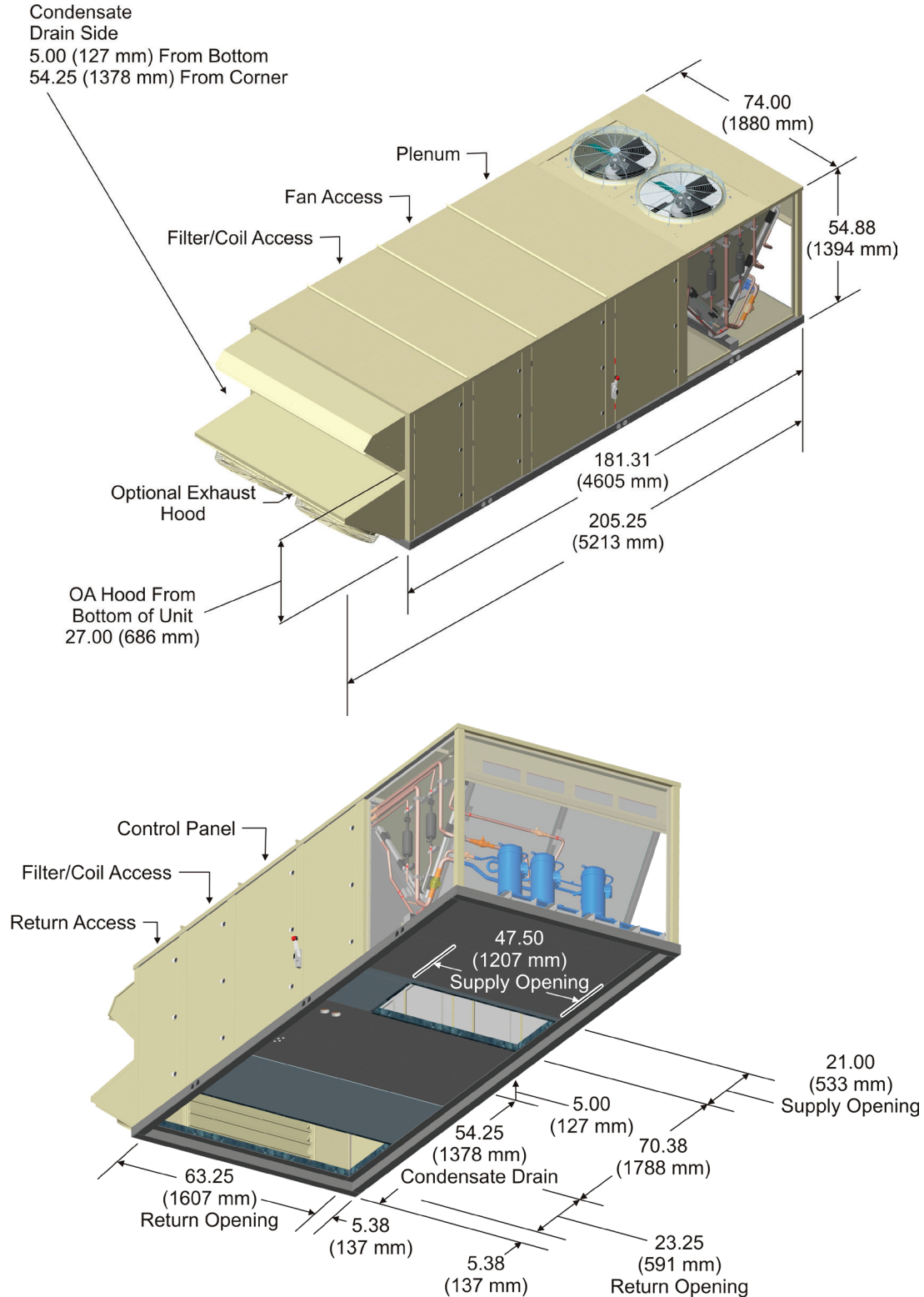
Figure 46: MPS 015–020 Cooling/Electric Heating Unit
