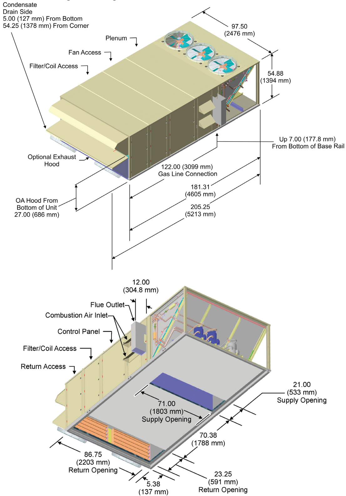
Figure 55: MPS 026–035 Cooling/Gas Heating Unit
