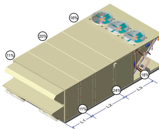
Figure 81: Weight Distribution Locations and % of Total Load (MPS 030–035 Example)
