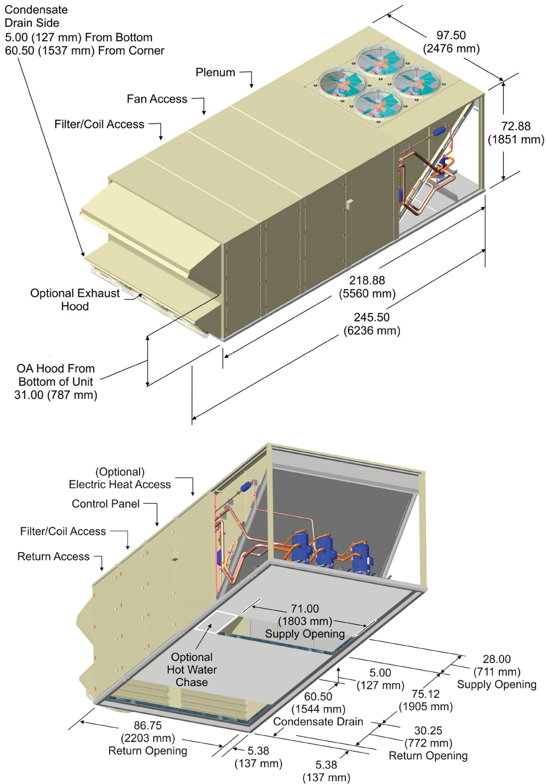
Figure 63: MPS 040–050 Cooling/Hot Water Heating Unit
