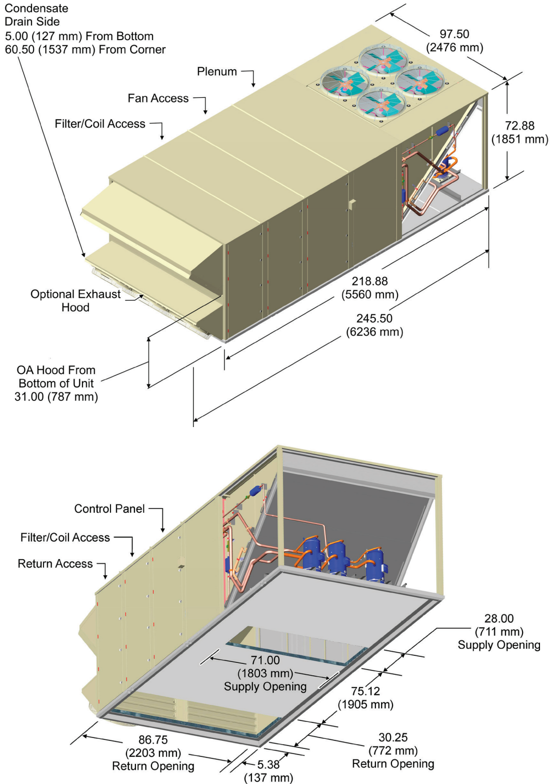
Figure 62: MPS 040-050 Cooling/Electric Heating Unit
